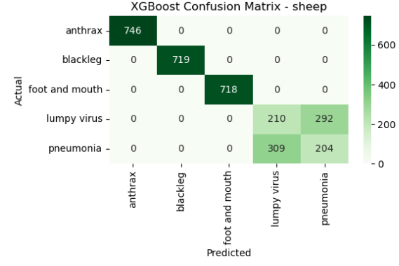
Figure 12: XGBoost confusion matrix - Sheep.
