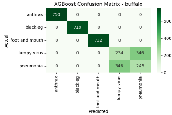
Figure 9: XGBoost confusion matrix - Buffalo.
