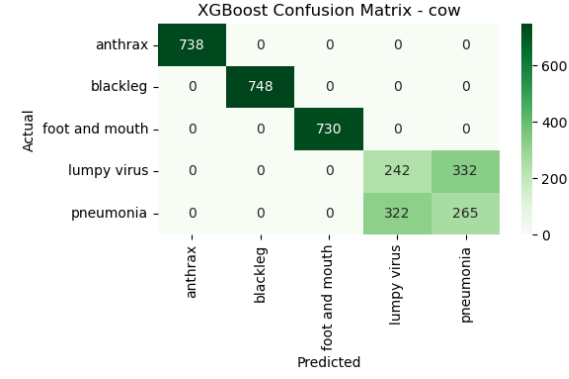
Figure 10: XGBoost confusion matrix - Cow.
