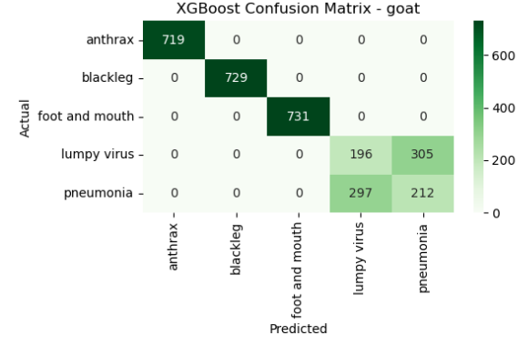
Figure 11: XGBoost confusion matrix - Goat.
