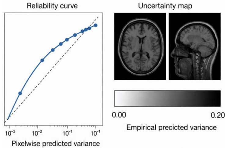
Figure 4: Uncertainty calibration and reliability plots.
