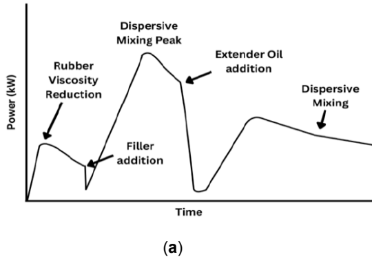
Figure 2: (a) Power/Time Curve (Mixing Cure observed in intermix), (b) NR/Conductive filler mixing in intermix. Sample- A, Sample-B, Sample-C, Sample-D.
